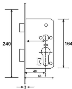
Roller Catch Lock For Both Side Opening Door
